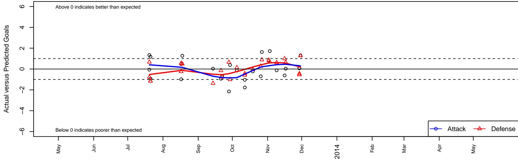
So Cal Blues Kale G00 Dots are actual minus expected GF (blue circles) and GA (red triangles). Blue line is smoothed change in attack strength. Red is smoothed change in defense strength.
